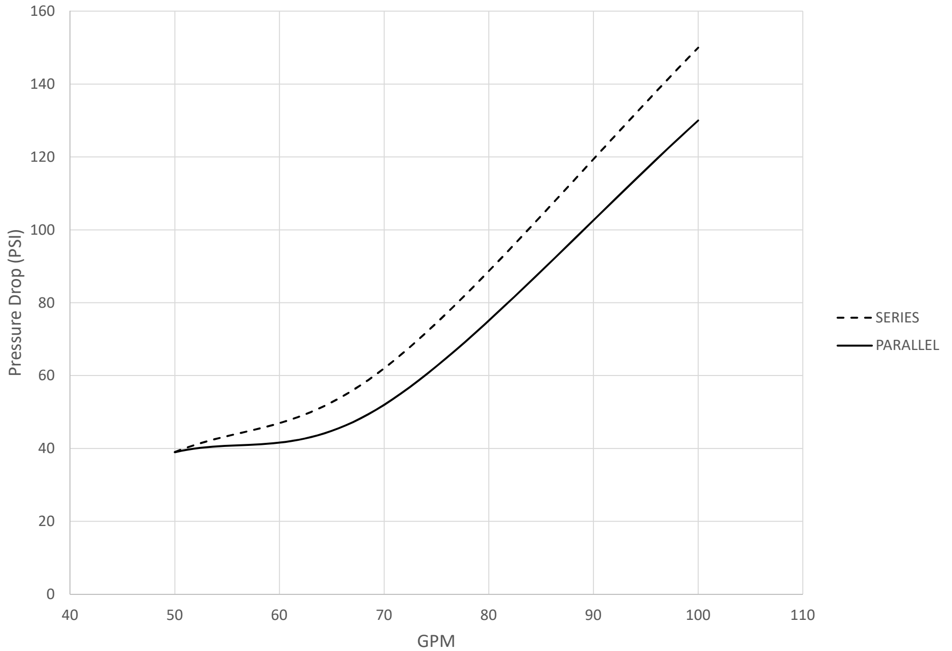
SP70HP Pressure Drop Curve
